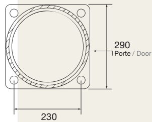
Semelle 4 tiges Base plate with 4 anchor bolts
