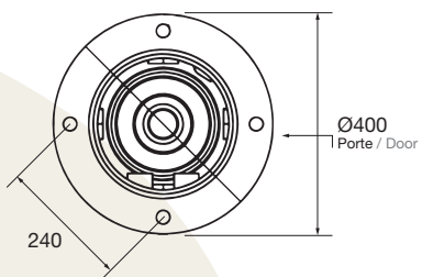
Semelle 4 tiges Base plate with 4 anchor bolts
