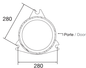
Semelle 3 tiges Base plate with 3 anchor bolts
